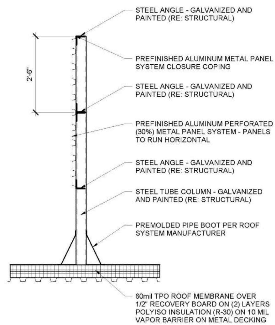
PROPOSED MECHANICAL SCREEN WALL DETAIL
